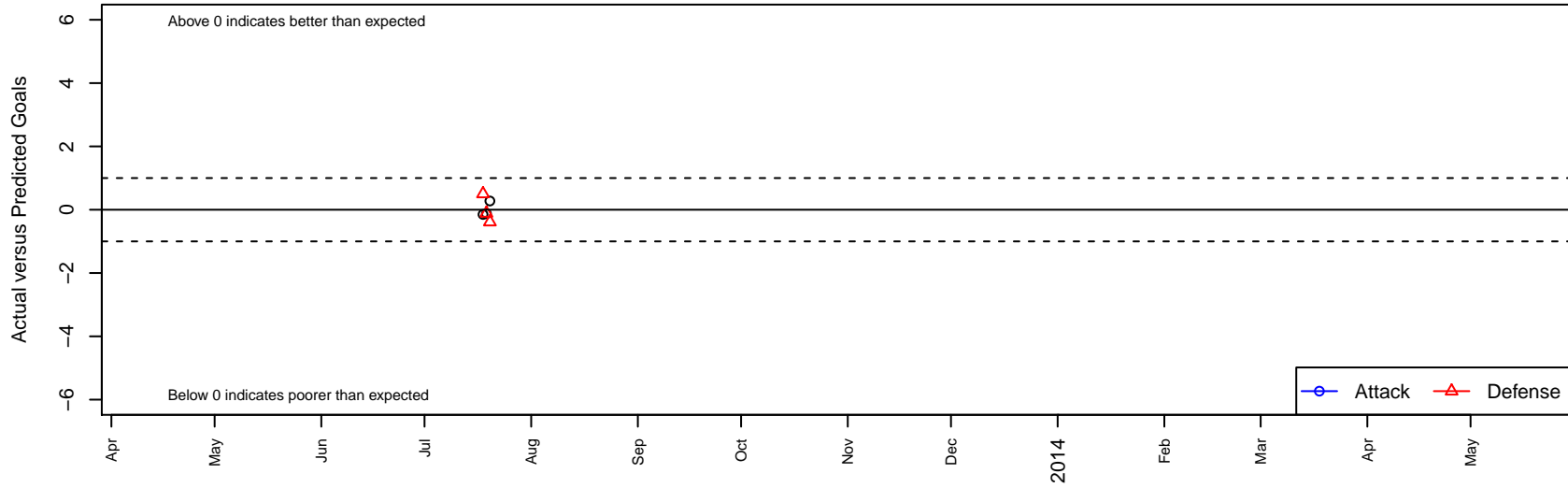
Dynamo Katner B96 Dots are actual minus expected GF (blue circles) and GA (red triangles). Blue line is smoothed change in attack strength. Red is smoothed change in defense strength.
